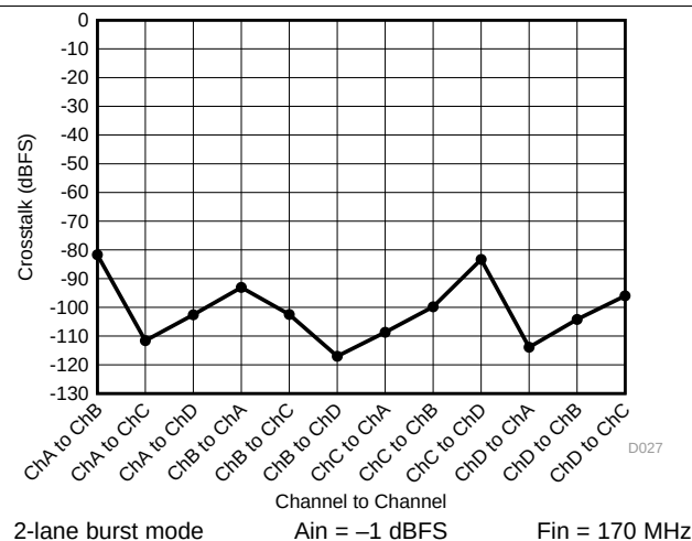
Figure 32. Burst Mode Crosstalk by Channel
