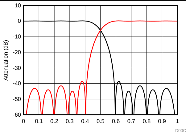
Figure 40. Decimation Filter Response
